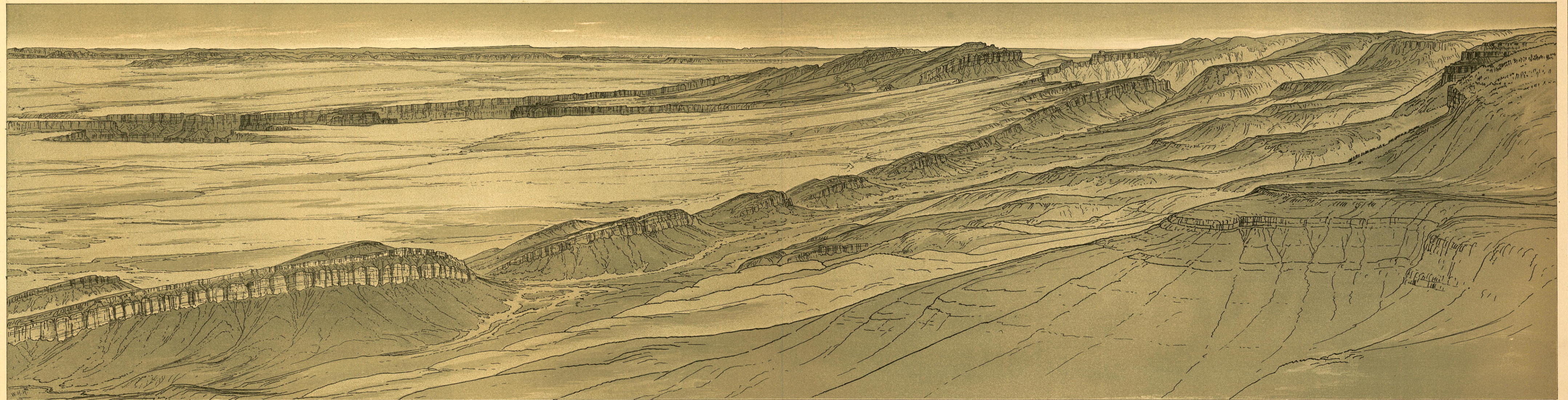
Upper View looking east-Lower View looking south-The two Views are continuous.The East Kaibab Monocline is immediately in front of the observer carrying the same geological horizon on which he stands down to the platform 2400 to 3000 feet below.
